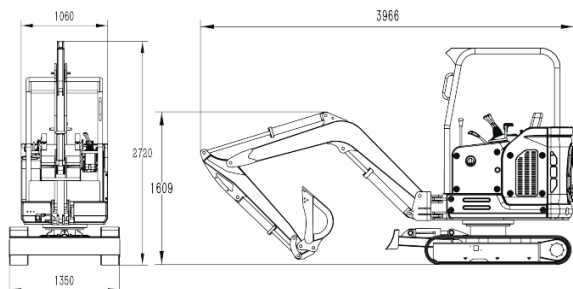
FRONT AND SIDE VIEW · DIMENSIONS IN MM
